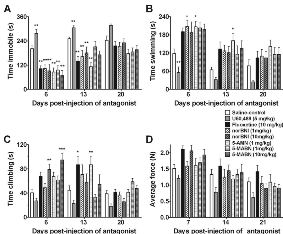
Figure 5. Effects of norbinaltorphimine, (norBNI) (1–10 mg/kg), 5'-(2-aminomethyl) naltrindole (5'-AMN) (1 mg/kg) and N-((Naltrindol-5-yl) methyl) pentanimidamide (5'-MABN) (1–10 mg/kg) on depression-related behavior in mice. (A) The time spent immobile, (B) swimming and (C) climbing during a 6 min forced swim test (FST) is shown. (D) In the tail suspension test (TST), a decrease in average force corresponds to increased immobility. Depression-related behaviors were measured in the same groups of animals on successive days following a single injection of antagonist, and 30 min after U50,488 (5 mg/kg) or fluoxetine (10 mg/kg) administration. Data are expressed as mean \pm standard error of the mean (SEM), n=10 per group. Comparisons to saline: * p<0.05 , ** p<0.01 , *** p<0.001
