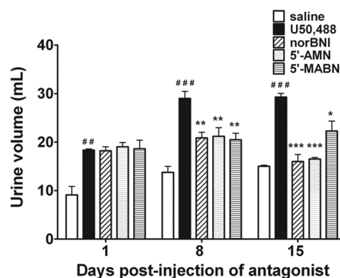
Figure 3. Antagonism of U50,488-induced diuresis in rats. Urine output over 4 h, following injection of U50,488 or saline (control) on test day, was measured on days 1, 8 and 15 post-injection of 1 mg/kg norbinaltorphimine (norBNI), 5'-(2-aminomethyl) naltrindole (5'-AMN), or N-((Naltrindol-5-yl) methyl) pentanimidamide (5'-MABN). Data are mean \pm standard error of the mean (SEM), n=4 per group. Comparisons to U50,488: * p<0.05 , ** p<0.01 , *** p<0.001 . Comparisons to saline: ## p<0.01 , ### p<0.001 .
