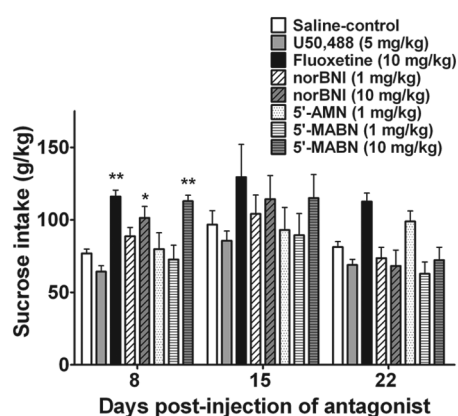
Figure 6. Effects of norbinaltorphimine, (norBNI) (1 and 10 mg/kg), 5'-(2-aminomethyl) naltrindole (5'-AMN) (1 mg/kg) and N-((Naltrindol-5-yl) methyl) pentanimidamide (5'-MABN) (1 and 10 mg/kg) on sucrose consumption in mice. Responses were measured at weekly intervals after a single injection of antagonist, and 30 min after U50,488 (5 mg/kg) or fluoxetine (10 mg/kg) administration. The mean \pm standard error of the mean (SEM) sucrose (5%) consumed in g of sucrose per kg body weight, during a 1 h test, is shown. n=10 per treatment group. Comparisons to saline: * p<0.05 , ** p<0.01
