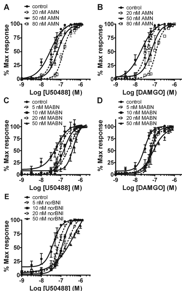
Figure 1. Cumulative concentration-response curves, in the isolated guinea-pig ileum for U50,488 and DAMGO, in the presence of increasing concentrations of (A) and (B) 5'-(2-aminomethyl) naltrindole (5'-AMN), (C) and (D) N-((Naltrindol-5-yl) methyl) pentanimidamide (5'-MABN), and (E) norbinaltorphimine (norBNI). All ligands tested caused rightward parallel shifts of agonist concentration-response curves. The results are expressed as the mean percentage of the maximum response induced by the agonist \pm standard error of the mean (SEM), n=4 tissues.
