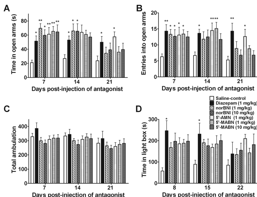
Figure 4. Effects of norbinaltorphimine, (norBNI) (1–10 mg/kg), 5'-(2-aminomethyl) naltrindole (5'-AMN) (1 mg/kg) and N-((Naltrindol-5-yl) methyl) pentanimidamide (5'-MABN) (1–10 mg/kg) on anxiety-related behavior in mice. (A) The time spent in open arms, (B) number of entries into the open arms and (C) total ambulation during a 5 min elevated-plus maze (EPM) test are shown. (D) The time spent in the lit compartment during a 10 min light dark box (LDB) test is also shown. Anxiety-related behaviors were measured in the same groups of animals on successive days following a single injection of antagonist, and 30 min after diazepam (1 mg/kg) administration. Data are expressed as mean \pm standard error of the mean (SEM), n=10 per group. Comparisons to saline: * p<0.05 , ** p<0.01 .
