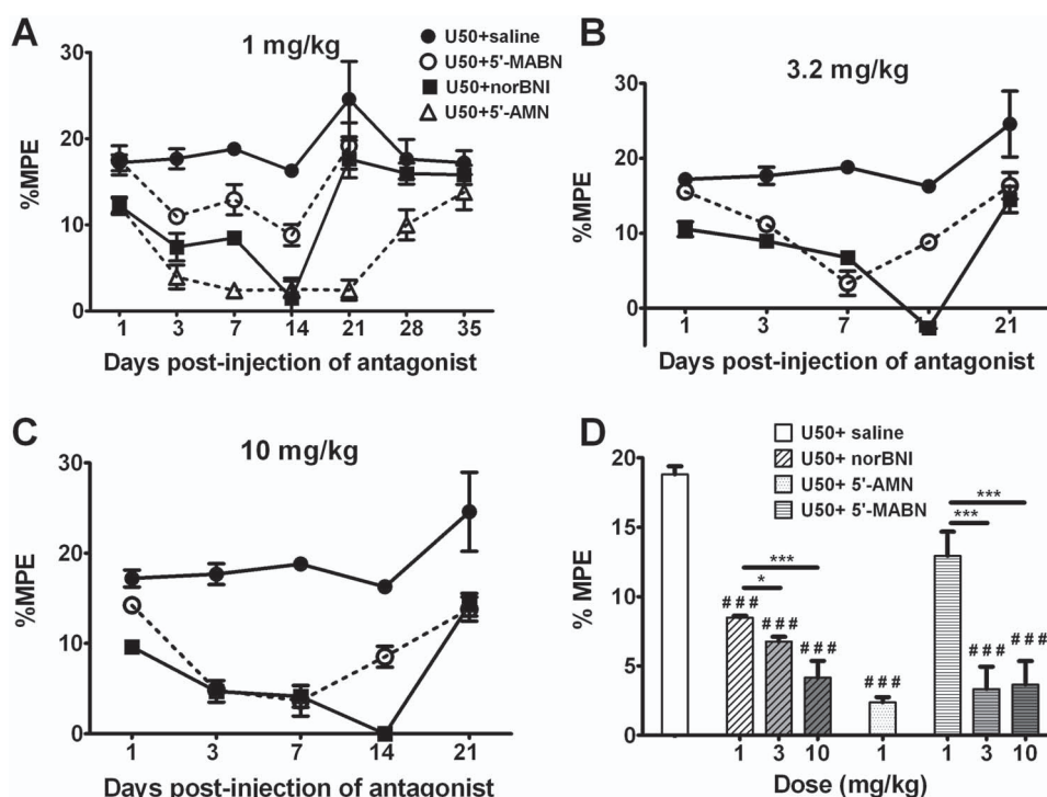
Figure 2. Ability of test compounds to block U50,488-induced antinociception in the tail-withdrawal test. Mice received a single injection of saline, norbinaltorphimine (norBNI), 5'-(2-aminomethyl) naltrindole (5'-AMN), or N-((Naltrindol-5-yl) methyl) pentanimidamide (5'-MABN) at doses of (A) 1 mg/kg, (B) 3.2 mg/kg or (C) 10 mg/kg and tail-withdrawal latency measured up to 35 days post-injection. (D) The data at seven days post-injection shows the dose-dependency of antagonism of U50,488-induced antinociception. Data are expressed as mean percentage maximum possible effect (%MPE) \pm standard error of the mean (SEM), n=4 to 8 per treatment group. Comparison to U50,488 + saline: ### p<0.001 . Comparison to 1 mg/kg test compound: * p<0.05 , *** p<0.001 .
